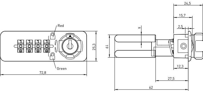
CODE 8002.021PN Combination lock Horizontal left 180° 1 x Clip
