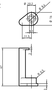
CODE 8002.C002 Cam
