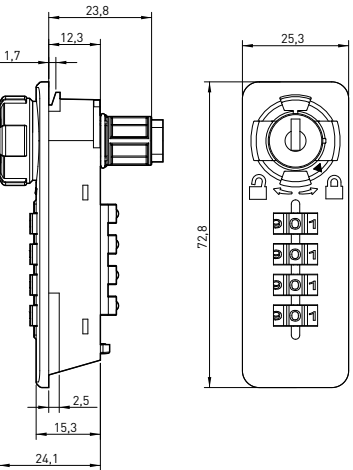
CODE 8002.001PN Combination lock Vertical right 90° 1 x Clip 1 x Screw L-8mm 1 x Loose cam
